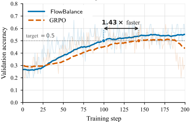
Training acceleration
